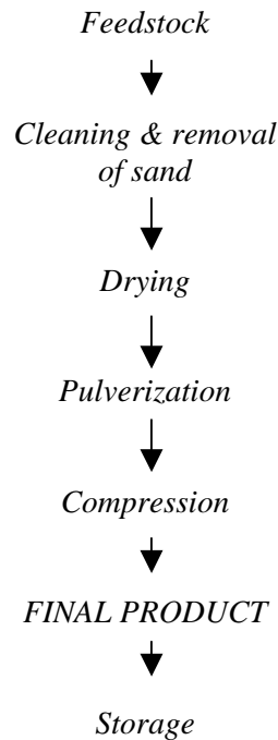
Figure 1. Flow diagram of the production process of briquettes from agricultural lignocellulosic residues (TDRI 1983).
